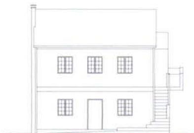
ALZADO PRINCIPAL
