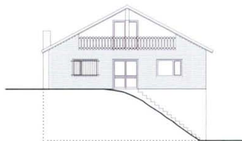
ALZADO PRINCIPAL
