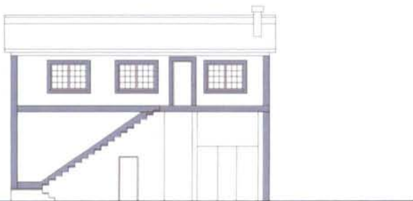
ALZADO PRINCIPAL
