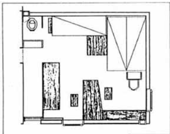
Petit Cabanon, plan of log cabin
